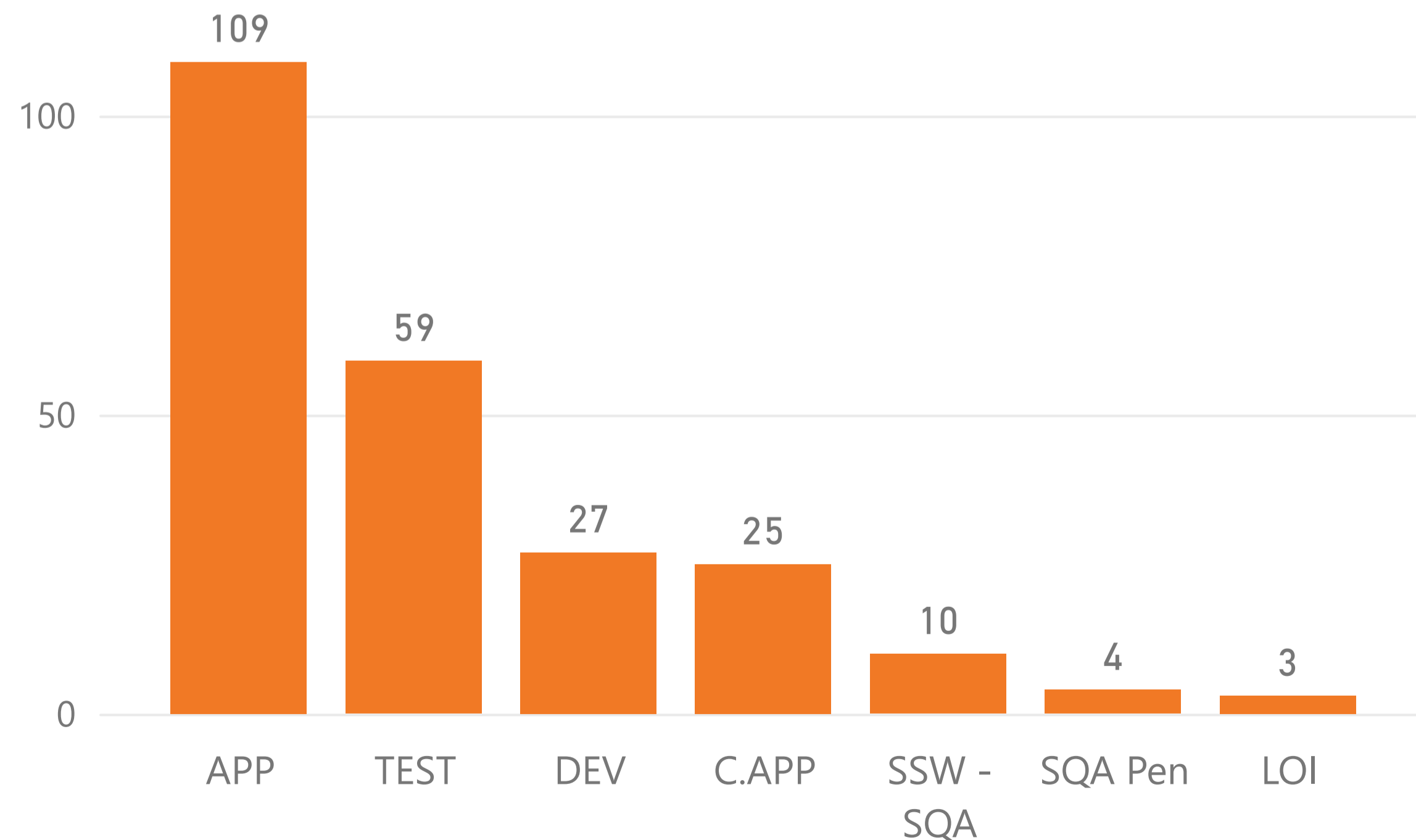
Total Beta dev parts by Part status
